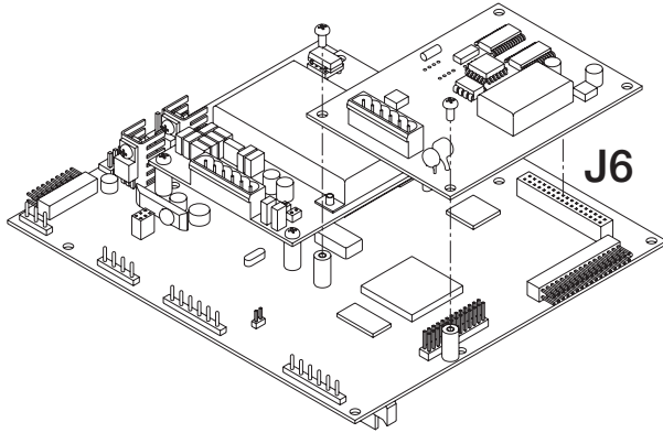
Figure 1. Installing Option Card Onto CPU Board
